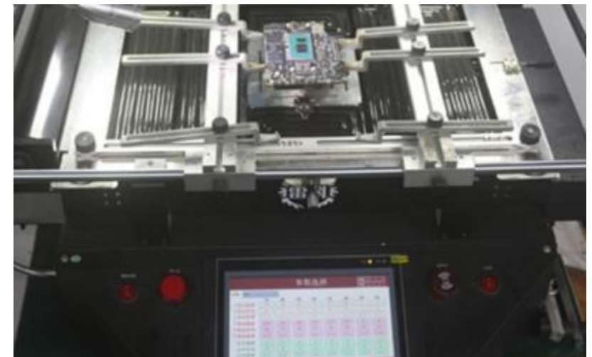
BGA Rework Station
