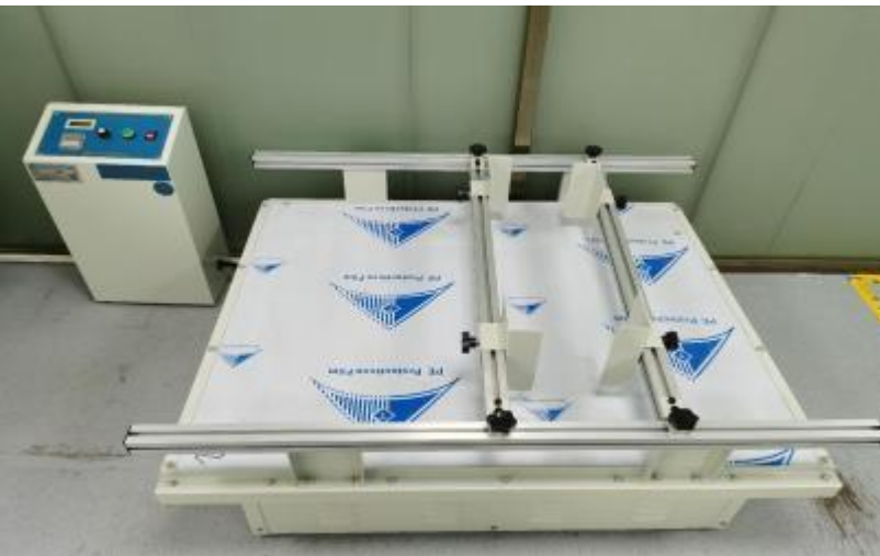
Simulated Transportation Shaker
